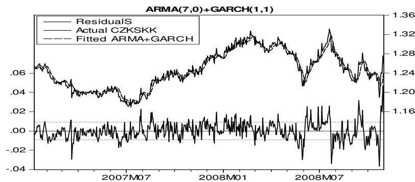
Figure 2: The estimated ARMA(7,0)+GARCH(1,1) model against the original datasets on whole range. (Residuals are at the bottom)
