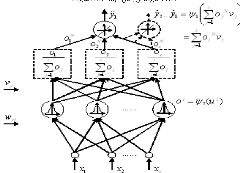
Figure 3: Soft (fuzzy logic) NN
