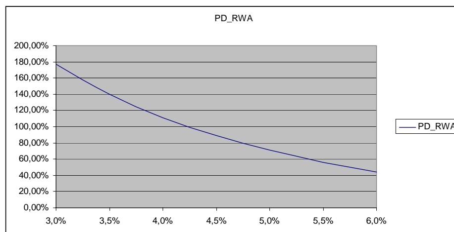
Figure 6 (99,9% PD-based Var Capital dependence on the definition of default)
