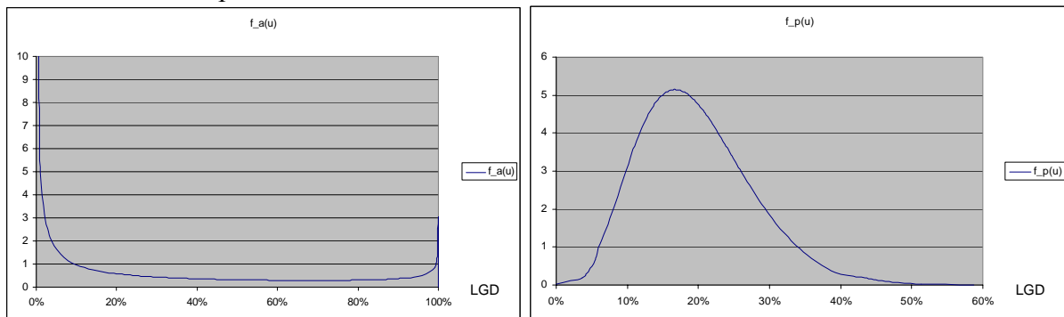
Figure 4 Account level beta distribution ( \mu=20\% and \sigma=30\% ) and its transformation into a portfolio distribution ( \rho=10\% )
