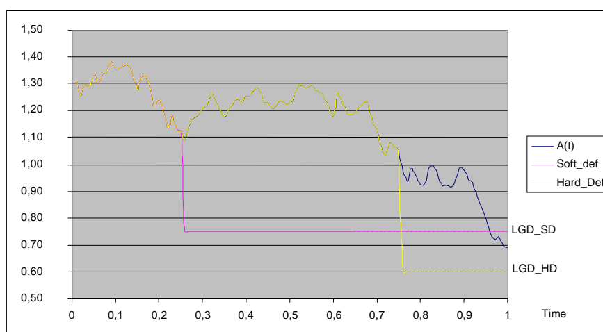
Figure 2 (Stochastic modeling of assets up to the time of default)
