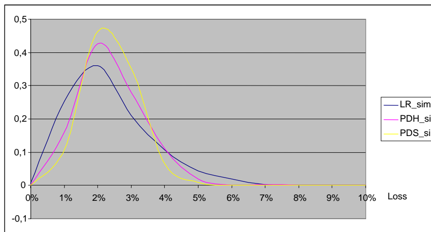
Figure 3 Histograms of simulated losses ( N=200, M=1000 )
