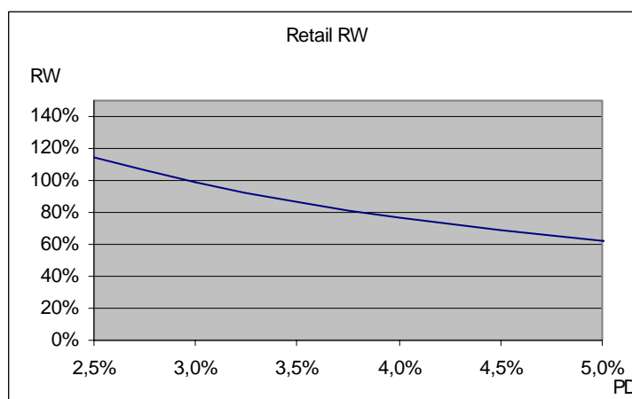
Figure 1 (Dependence of regulatory RW=12,5 \cdot C on PD )
